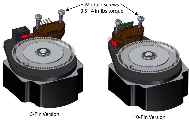
10-Pin Version
